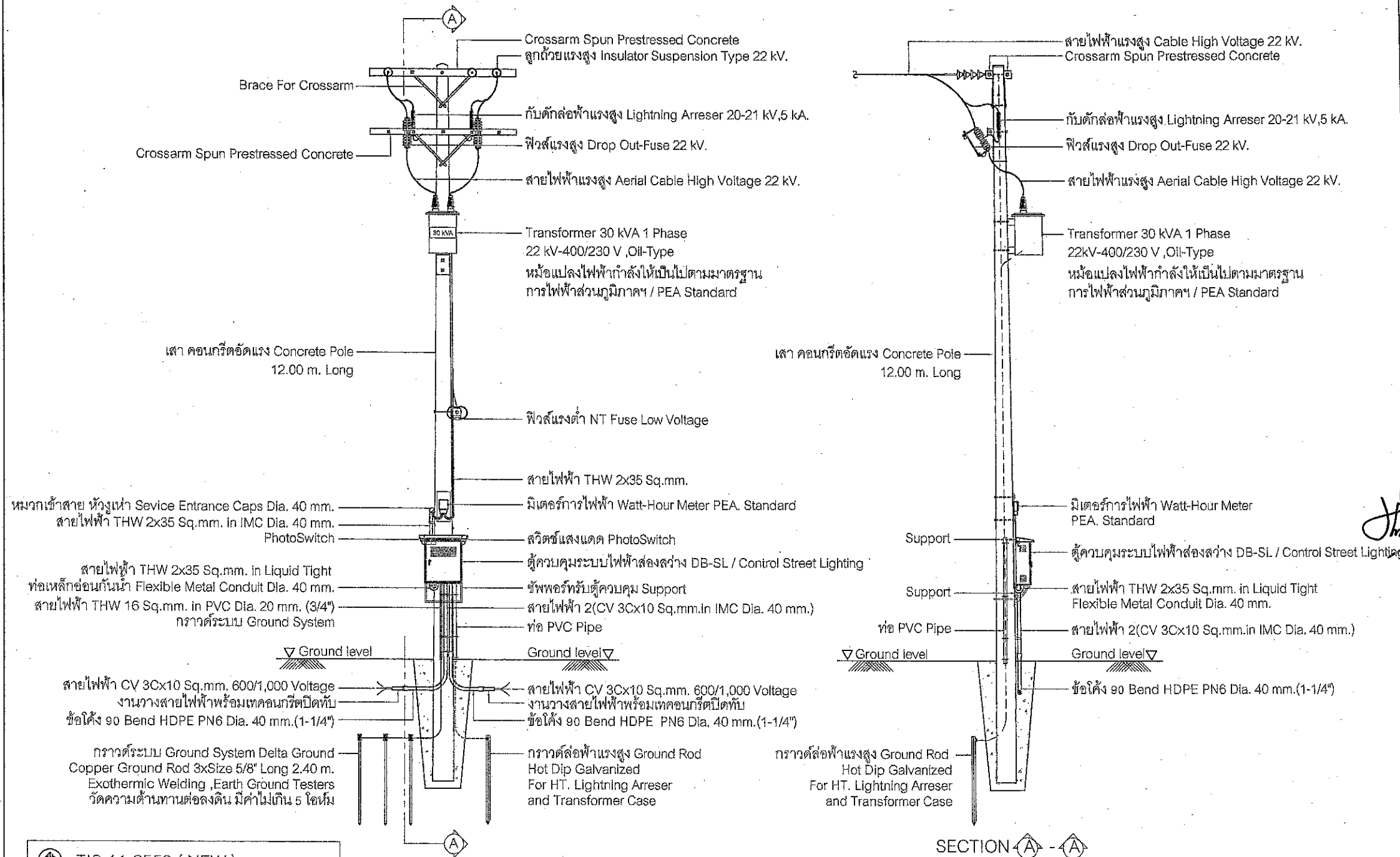
Detail "Transformer 30 kVA & DB-SL Control Street Lighting"
